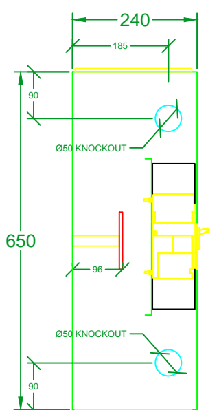
SIDE VIEW (TOBLNT.00/160CB)
