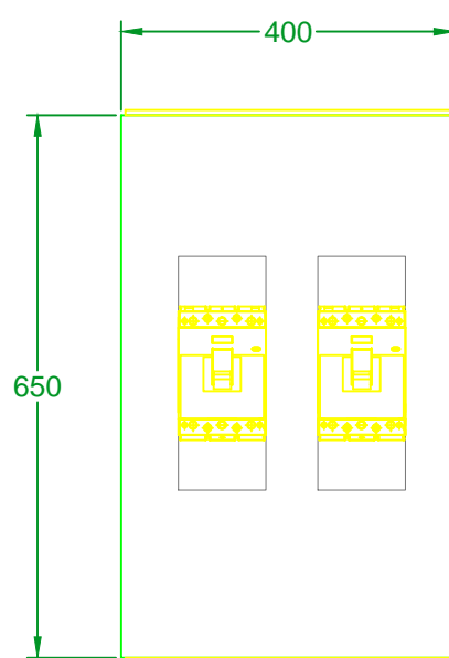
FRONT VIEW (TOBLNT.00/160)
