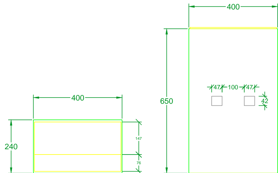
TOP/BOTTOM VIEW (ALL)
