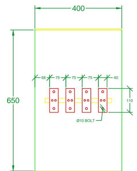
FRONT VIEW (EOR ONLY) (BEHIND DIN FUSE DISCONNECTOR) (TOBLNT.00/160EOR)
