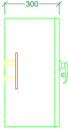
SIDE ELEVATION
