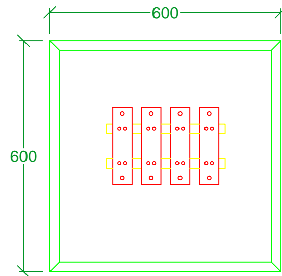
FRONT ELEVATION
