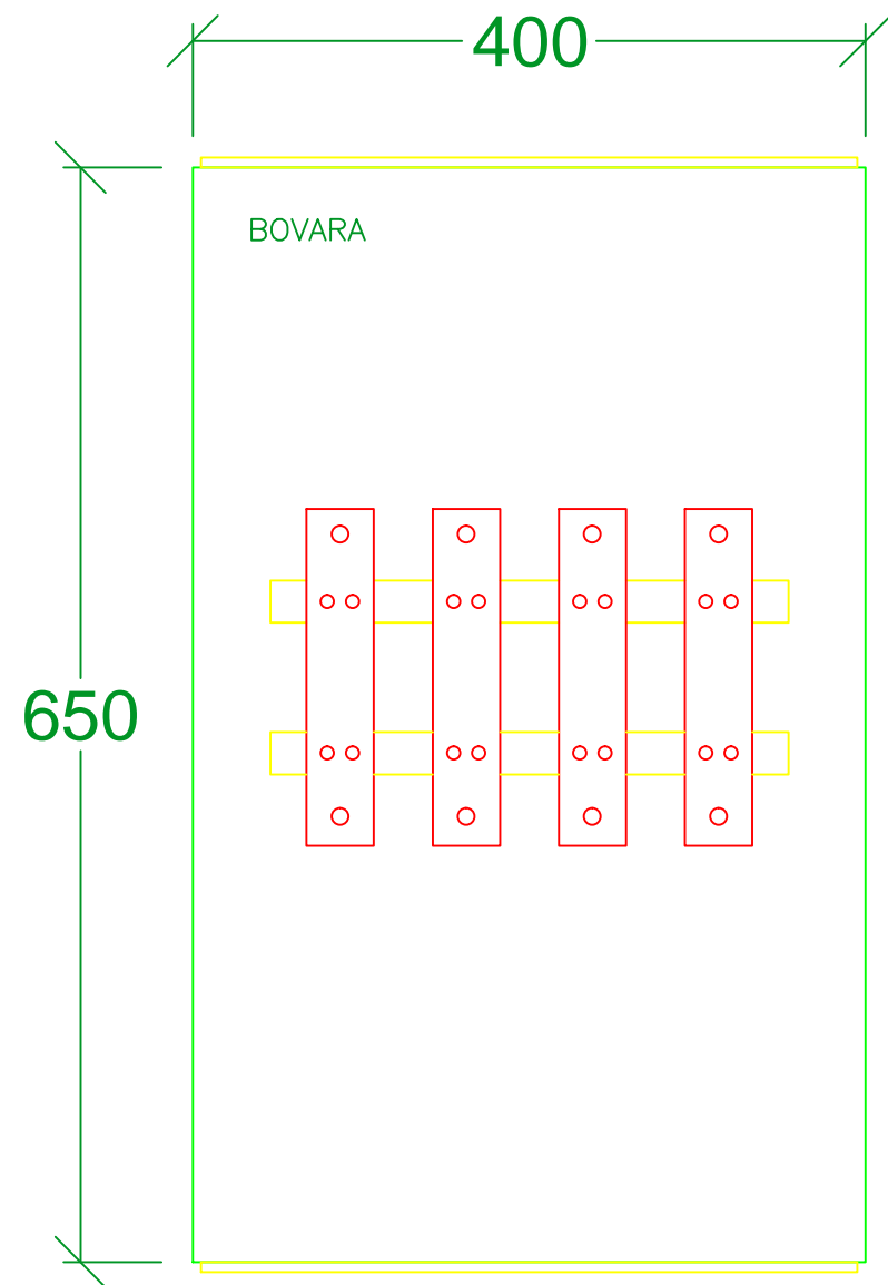
FRONT ELEVATION
