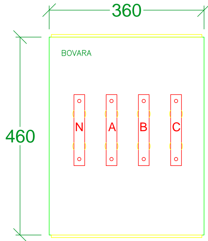
FRONT ELEVATION
