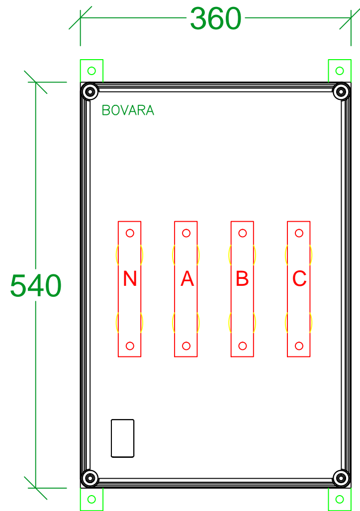
FRONT ELEVATION
