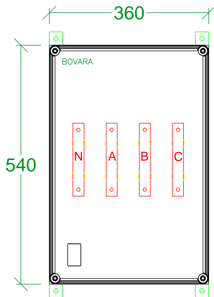
FRONT ELEVATION
